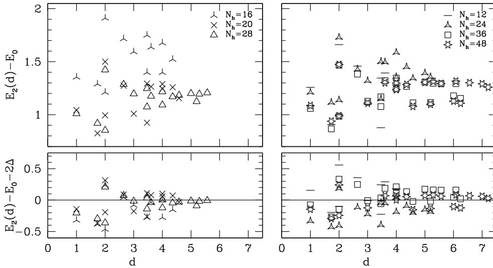
Figure 3. The energy E_2(d) of the ground state of the \mu QDM in the presence of two holes at distance d . In the top panels this energy is compared to the energy E_0 of the system without holes and in the lower panels E_2(d) is compared to the hole-free energy E_0 corrected by twice the energy cost \Delta = E_1 - E_0 of a single hole.
