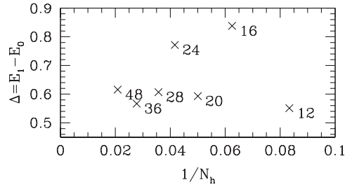
Figure 2. The energy cost \Delta of a single hole in the \mu QDM as a function of the number of hexagons N_h .
