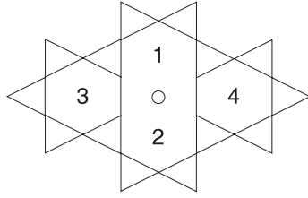
Figure 1. The hole forbids all resonance loops on hexagons 1 and 2 and suppresses some of the loops around 3 and 4.
